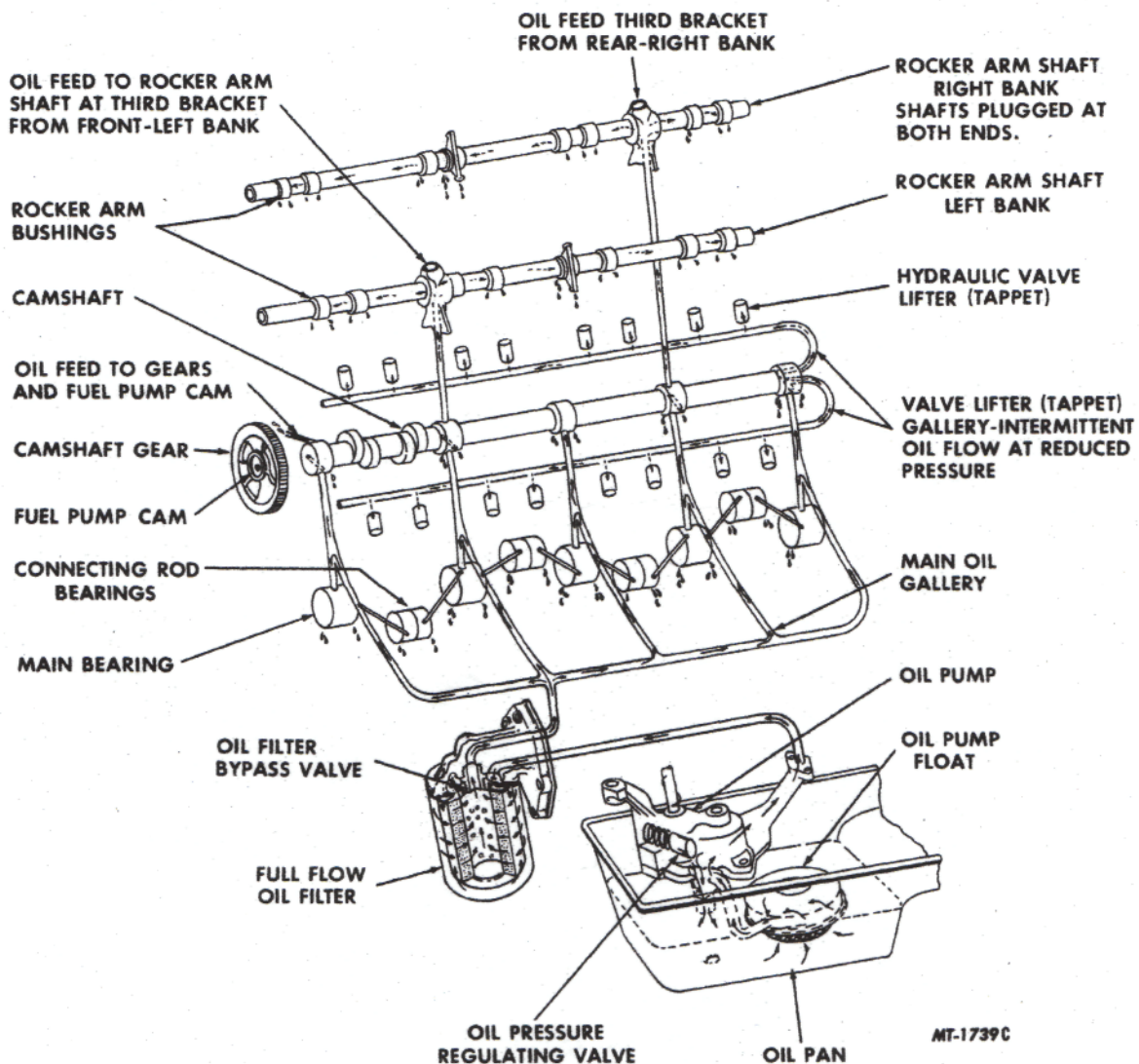
Fig. 5 Diagrammatic View of Lubricating System
